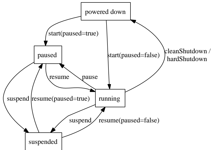
Figure 1.1: VM Lifecycle
