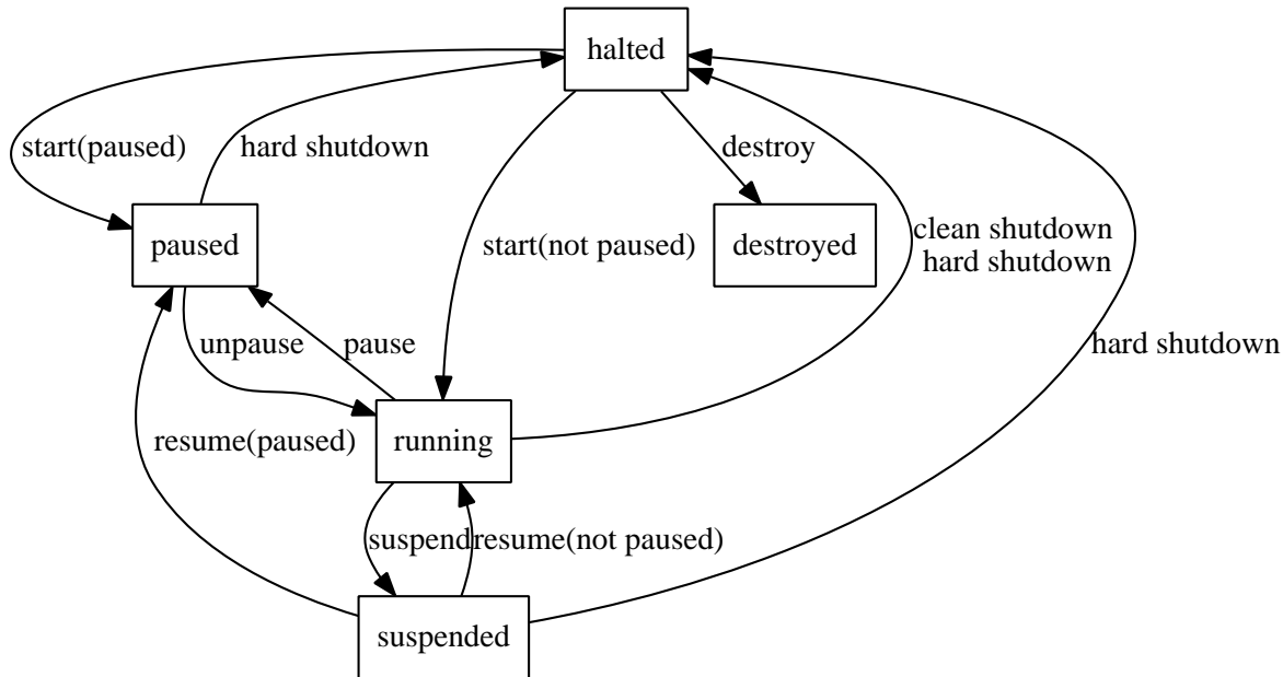
Figure 1.1: VM Lifecycle
