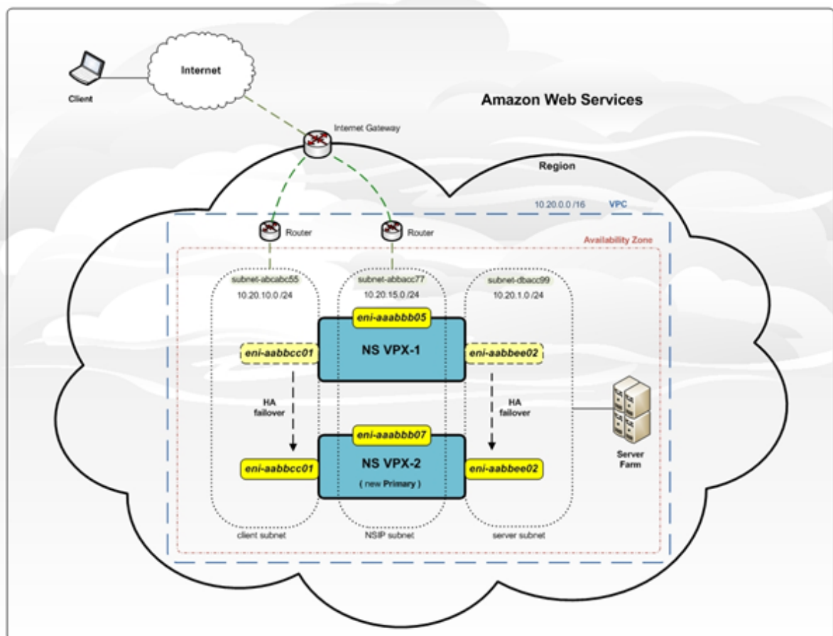
Figure 1. A NetScaler VPX HA Pair on AWS
