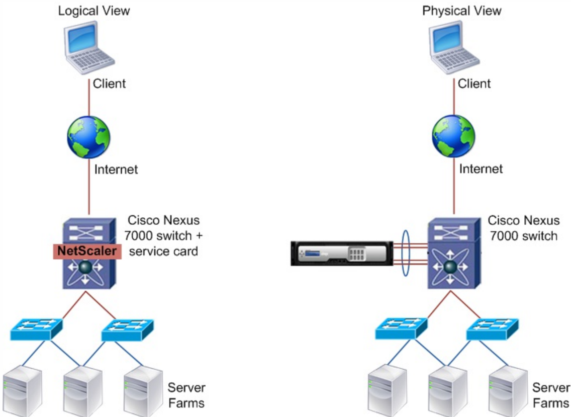
Figure 1. RISE Deployment
