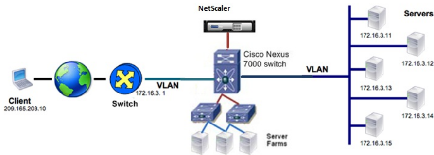
Figure 3. Bridged Mode
