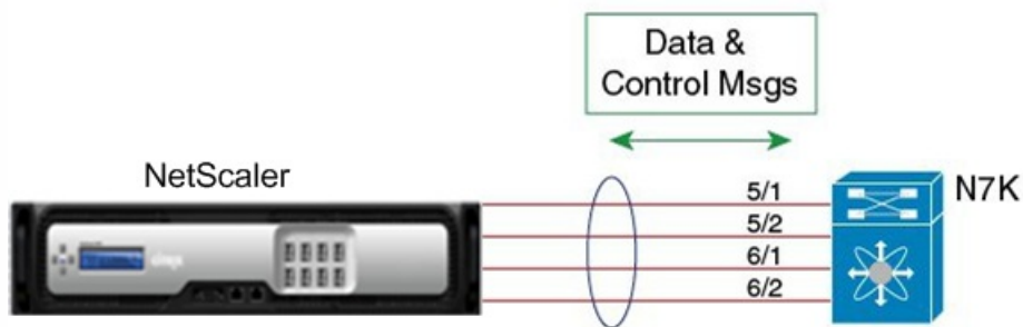
Figure 5. Direct Connect Mode
